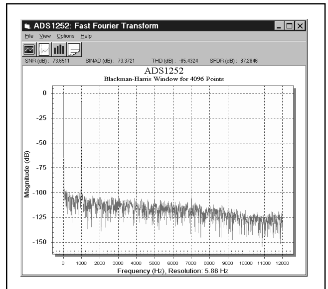
FIGURE 6. FFT Display.
